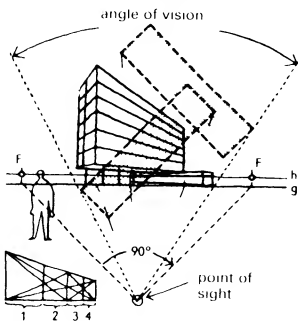
14 Perspective method
